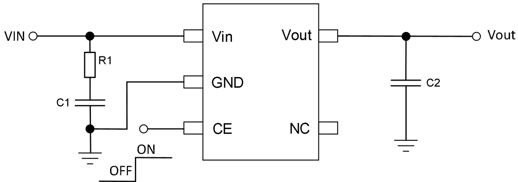
Figure 2 Hot Plug application circuit
