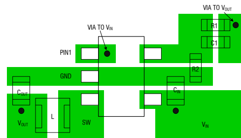
Figure 3. XR3406Suggested Layout
